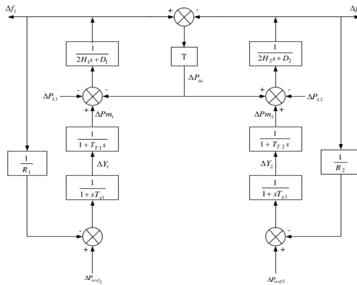
FIGURE 1. LFC System Two Area [11]
