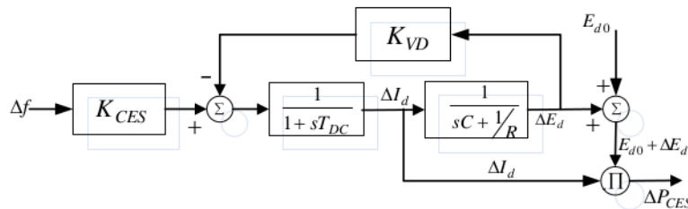
FIGURE 3. Capacitive energy storage block diagram
