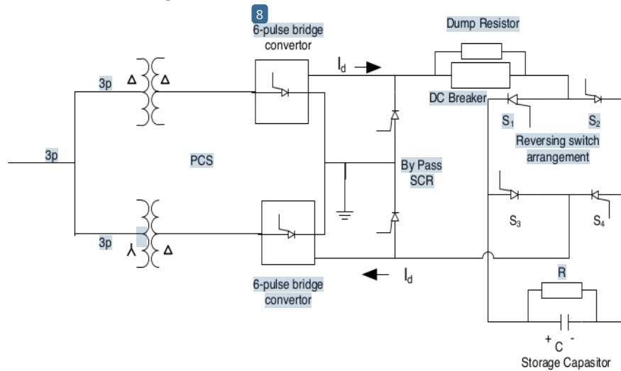
FIGURE 2. Capacitive energy storage
