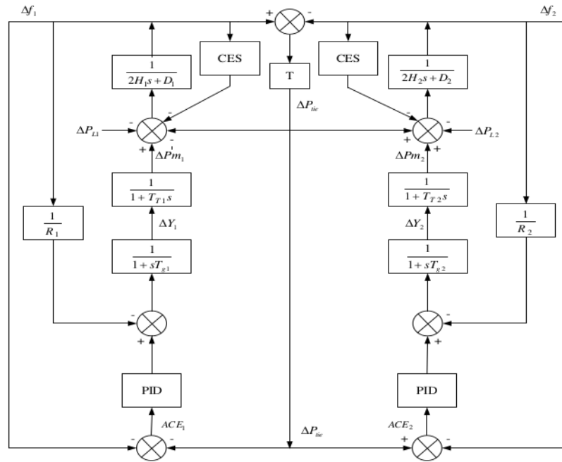
FIGURE 4. Systems with PID and CES controllers
